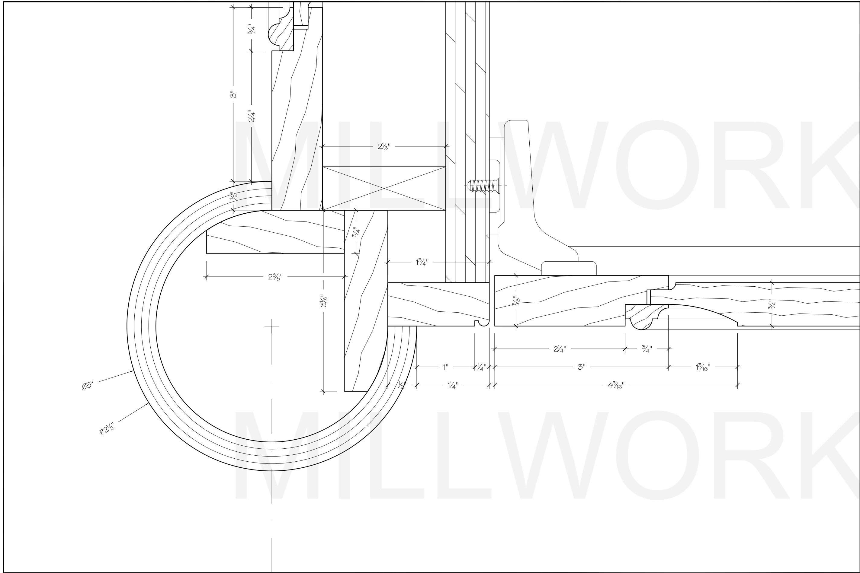
6 SECTION DETAILS SCALE: FULL CORNER COLUMN GUEST BATH
