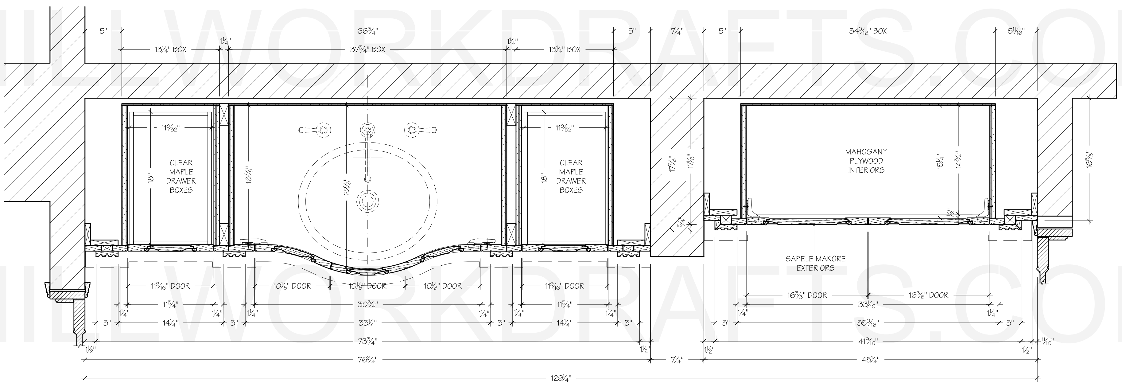
SECTION PLAN 1 VANITY AND LINEN CLOSET SCALE: 1-1/2" = 1'-0" DAVID'S BATH
