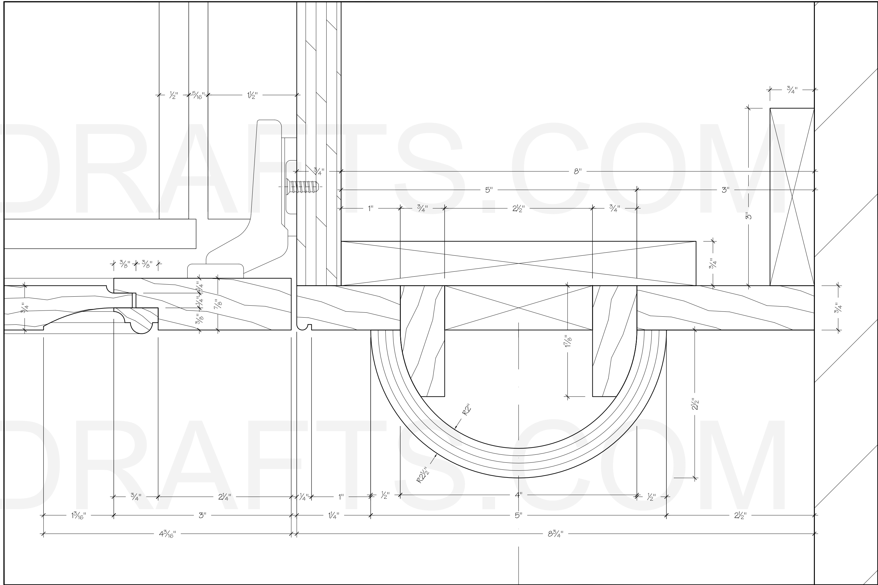
7 SECTION DETAILS SCALE: FULL SIDE COLUMN GUEST BATH
