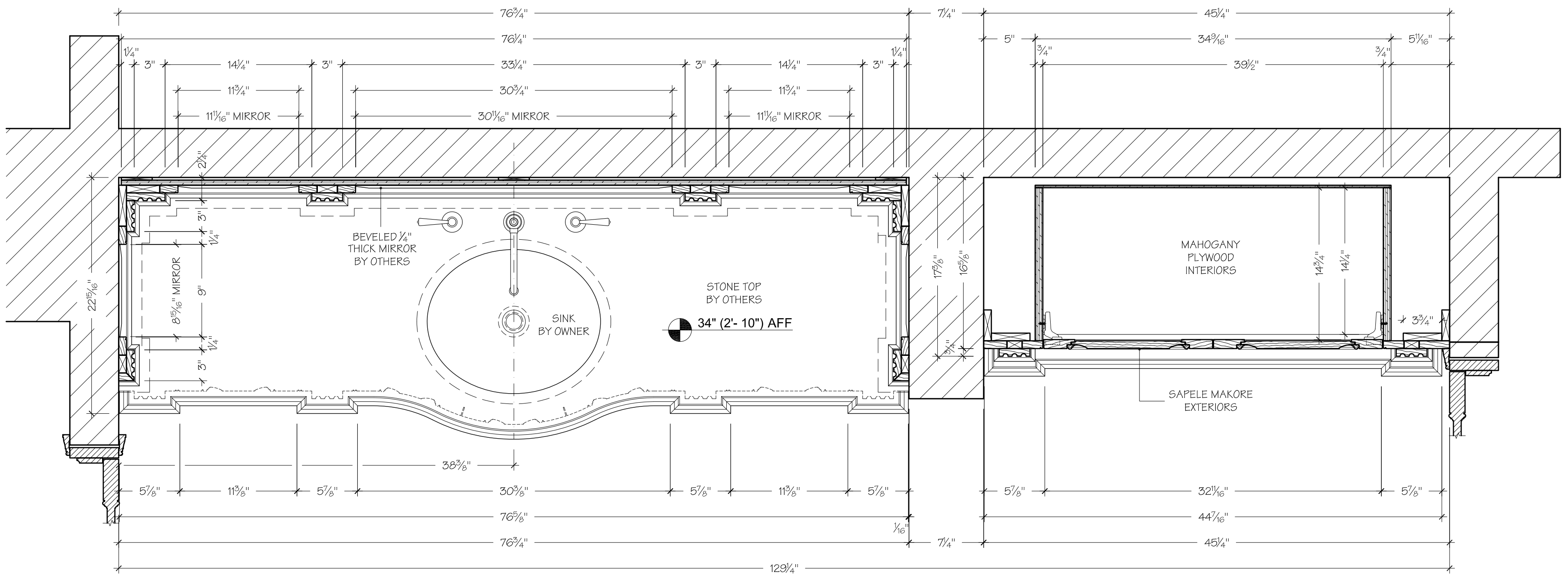
SECTION PLAN 2 VANITY AND LINEN CLOSET SCALE: 1-1/2" = 1'-0" DAVID'S BATH
