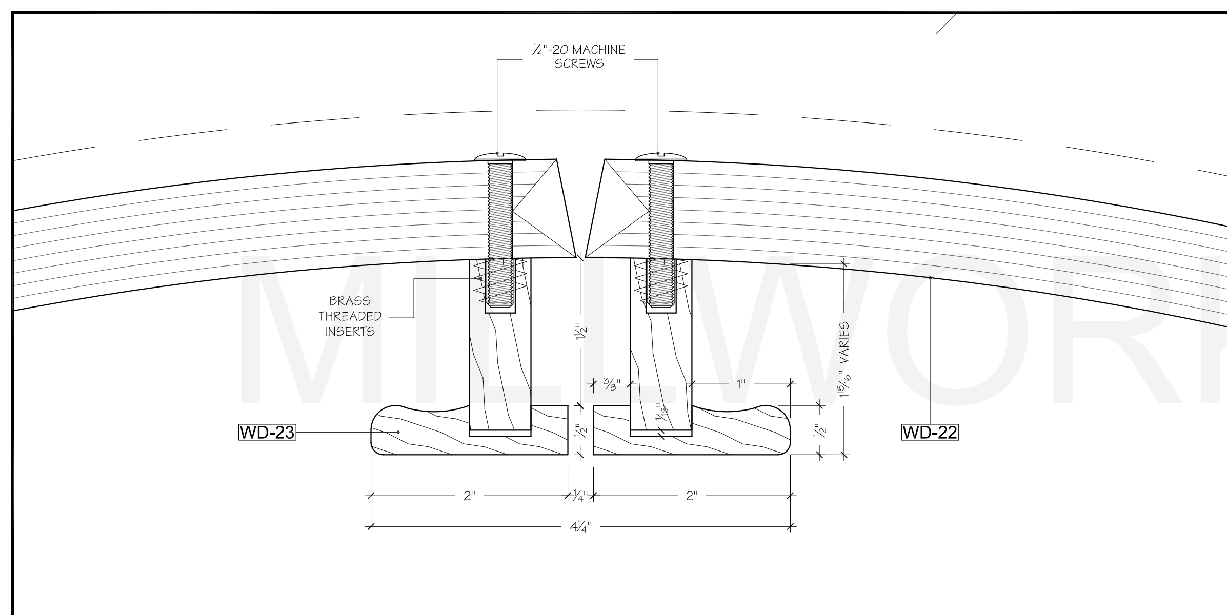
10 SECTION DETAILS SCALE: FULL
