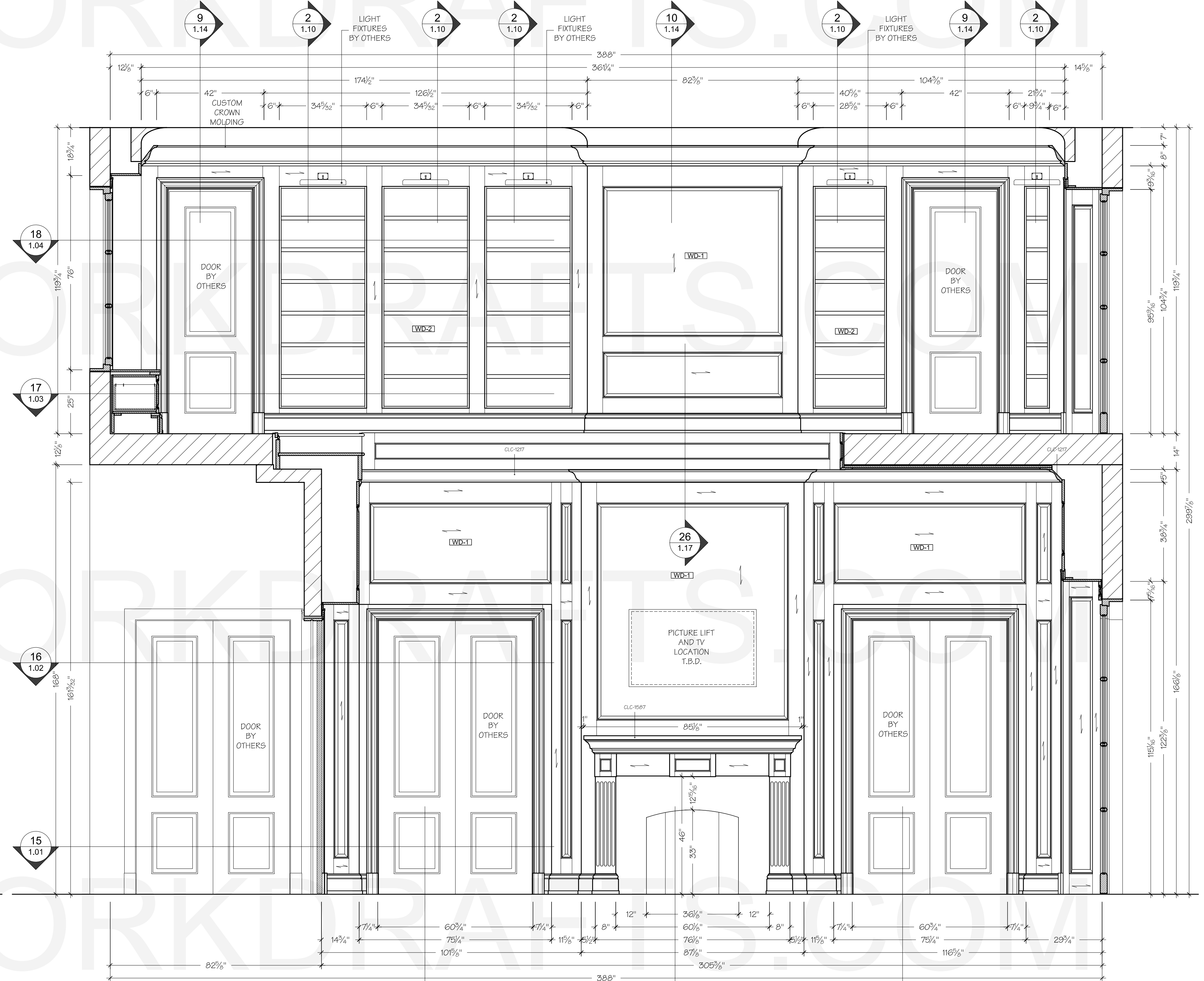
C ELEVATION SCALE: 1/2" = 1'-0" LIBRARY & MEZZANINE
