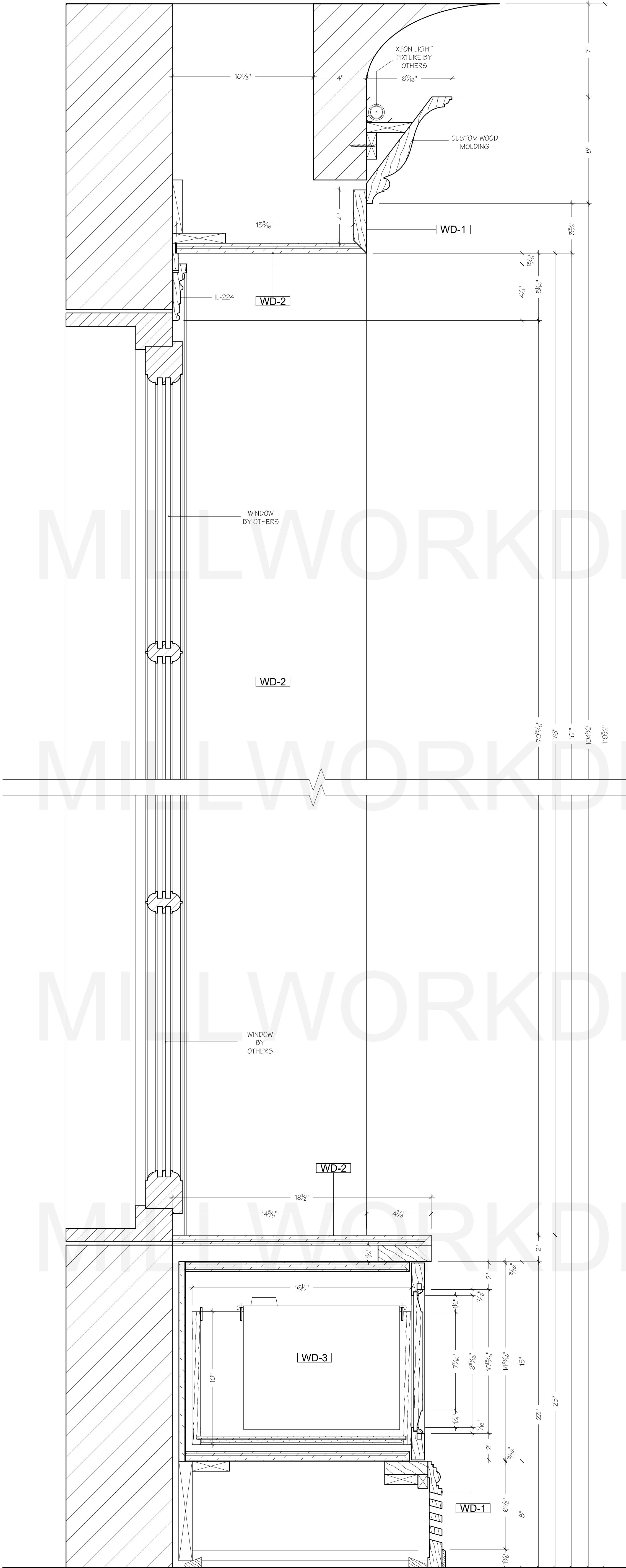
3 SECTION WINDOW SEAT & STORAGE DRAWER MEZZANINE SCALE: 3" = 1'-0"
