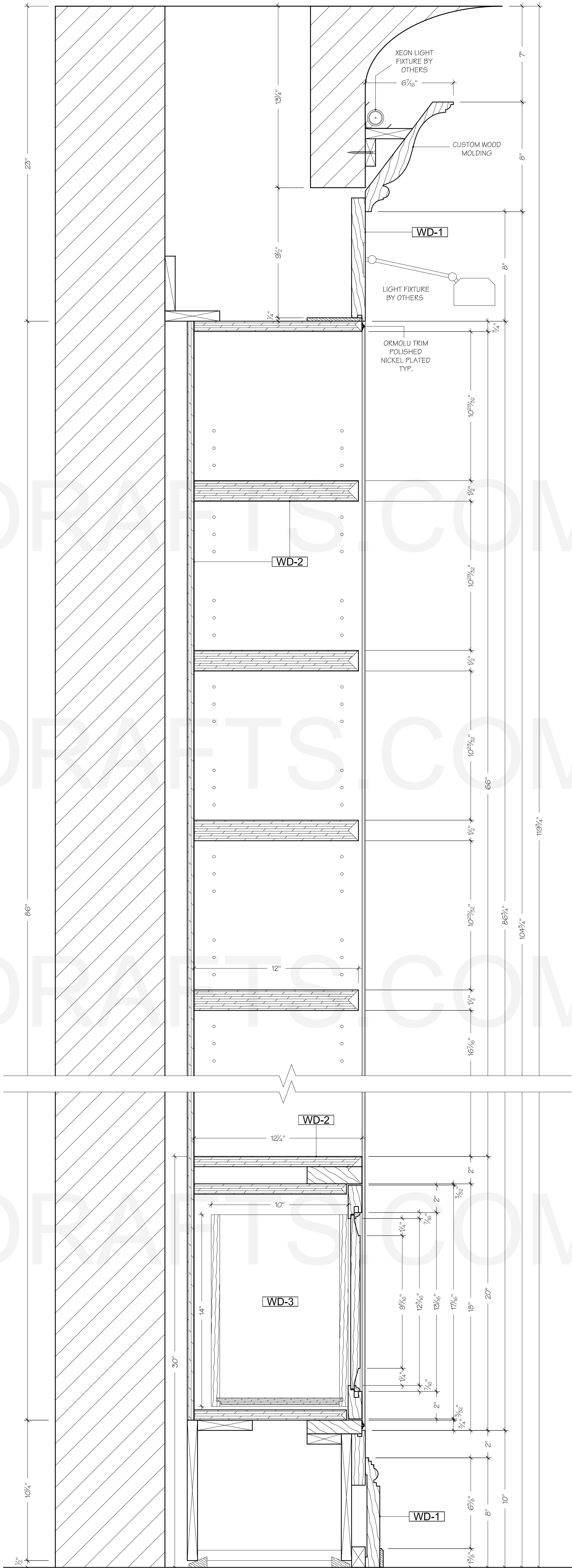
6 SECTION SCALE: 3" = 1'-0" STORAGE DRAWER & BOOK SHELVES MEZZANINE
