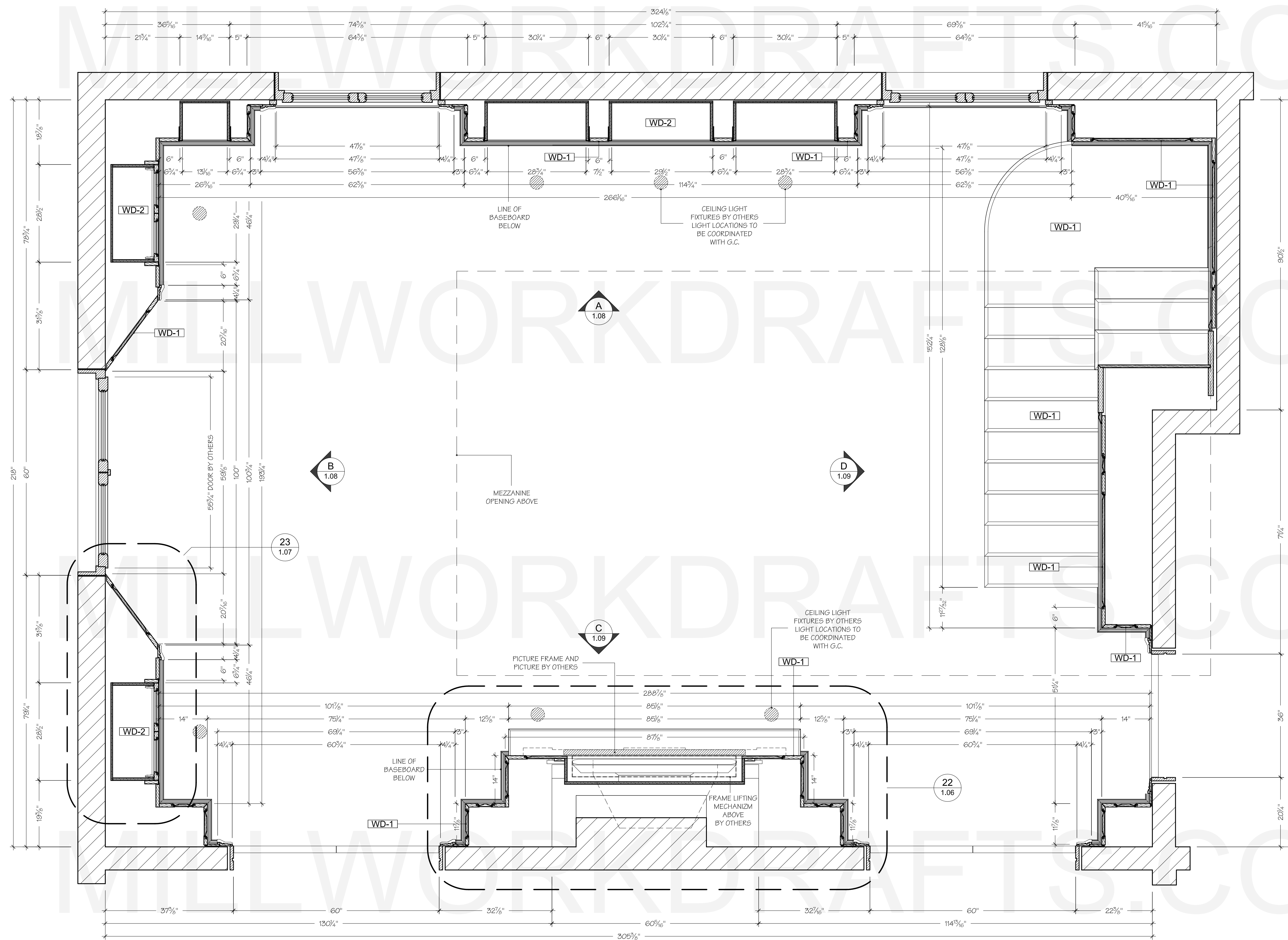
SECTION PLAN SCALE: 3/4" = 1'-0" LOWER LEVEL LIBRARY
