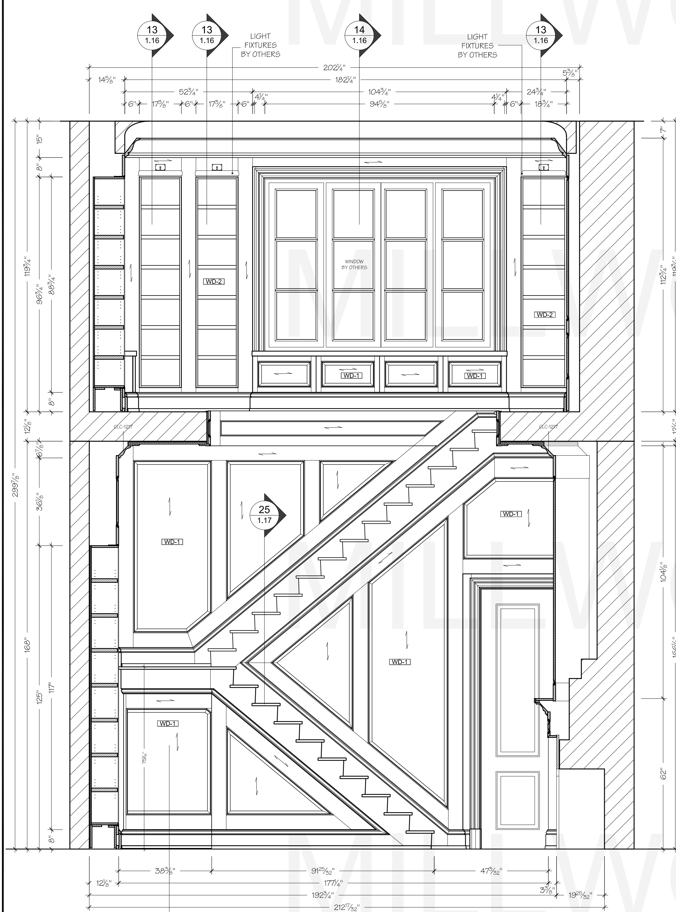
D ELEVATION SCALE: 1/2" = 1'-0" LIBRARY & MEZZANINE
