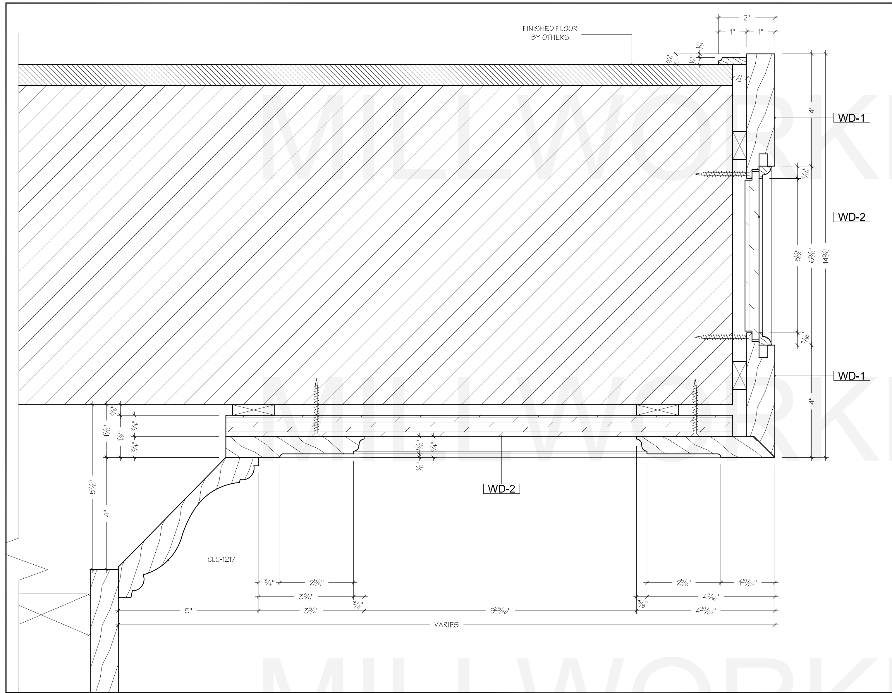
25 SECTION DETAILS @ MEZZANINE FREEZE & CEILING PANELS SCALE: HALF LIBRARY
