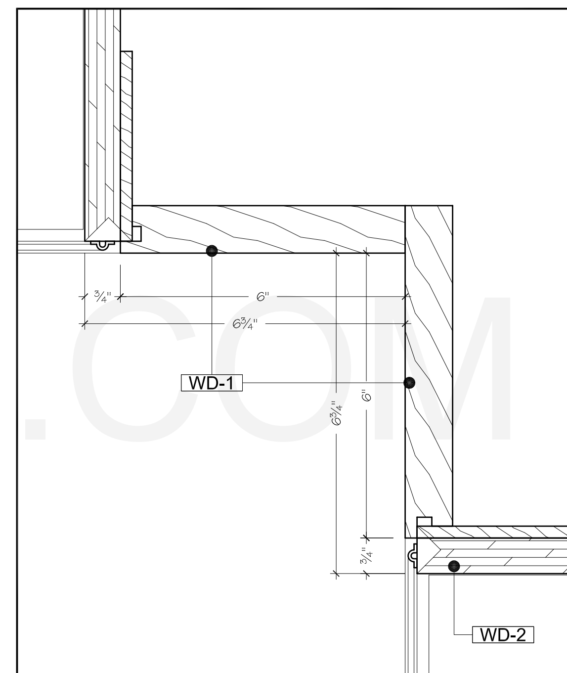
30 SECTION DETAILS TYPICAL CABINET CORNER PILASTERS SCALE: HALF LIBRARY
